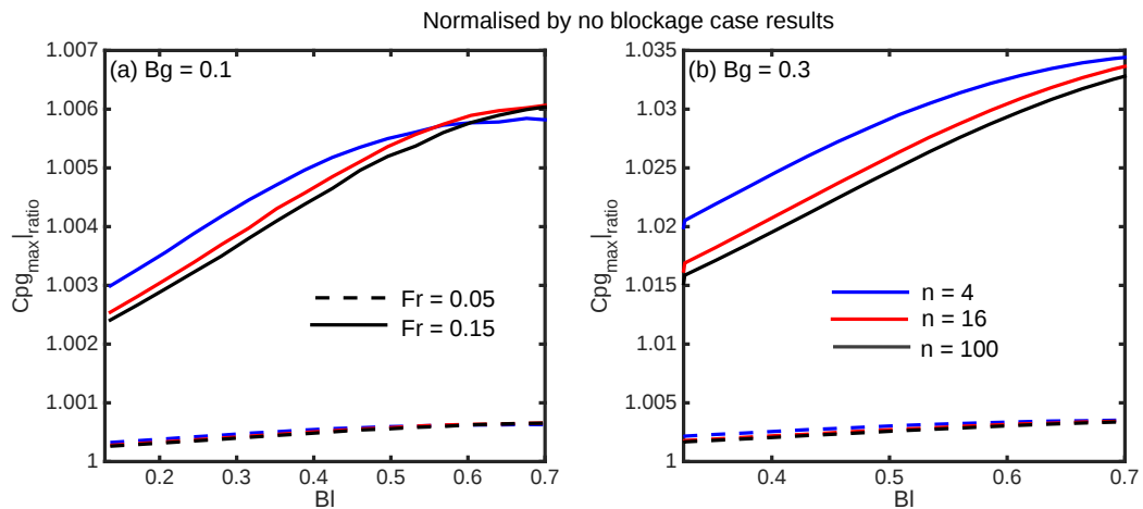
Figure 2: The optimal global power coefficient normalised by the corresponding optimal power coefficient in the cases with no free-surface deformation ( Cpg_{max|ratio} ) are presented for (a) Bg = 0.1 and (b) Bg = 0.3 . It is seen that the increment in the power coefficient caused by the free-surface deformation effects increase with Bl , and that this increment is usually higher in the farms with a fewer number of turbines.
