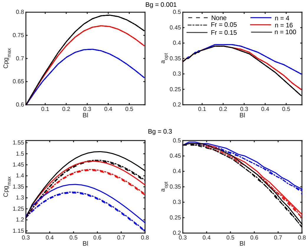
Figure 1: The left and right plots present the results for the maximum global power coefficient Cpg_{max} and the corresponding optimal induction factors ( a_{opt} ), respectively, as functions of the local blockage ratio Bl . The top plots are for a low blockage case Bg = 0.001 , and the bottom plots are for a high blockage case Bg = 0.3 . The results are presented for farms with different number of turbines and Froude number as shown by the markers in the top right plot. As expected the free-surface deformation effects are not observable in the Bg = 0.001 case, and in the Bg = 0.3 case these effects increase with the Froude number. Cpg_{max} increases with the increase in Bg and Fr . Bl and a_{opt} corresponding to the maximum in Cpg_{max} also increase slightly with Fr .
