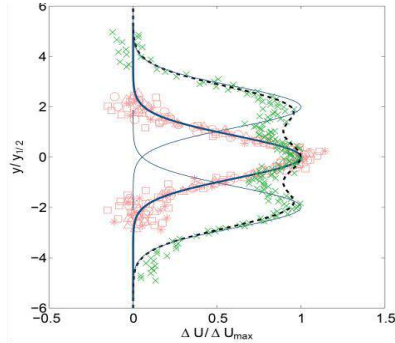
Fig. 1: Transverse profile of normalized velocity for experimental study of a single rotor wake, at X = 4D(\Delta) , 6D(\circ) , 8D(\square) and 10D(*) with self-similar Gaussian profile ( \text{—} ) and 6D downstream of a fence of 3 rotors ( \times ), with single wakes ( \text{—} ) and superposition ( \text{--} ).
