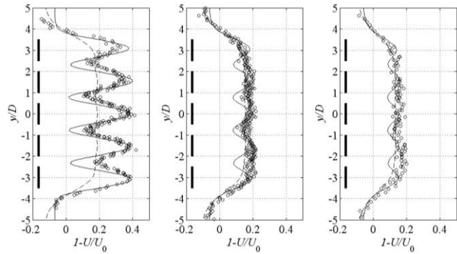
Fig. 2: Transverse profiles of velocity deficit for a single row of 5 rotors at 1.5D lateral spacing by superposition ( \text{--} ), RANS-BEM ( \text{—} ) and experiment ( \circ ) for X = 4D (left), 8D (centre) and 10D (right) downstream. Rotor plane ( \text{—} ).
