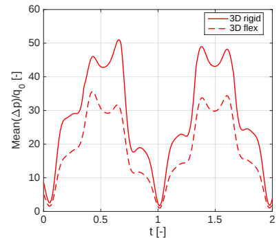
Fig. 6. Computed \Delta p rotating blade
