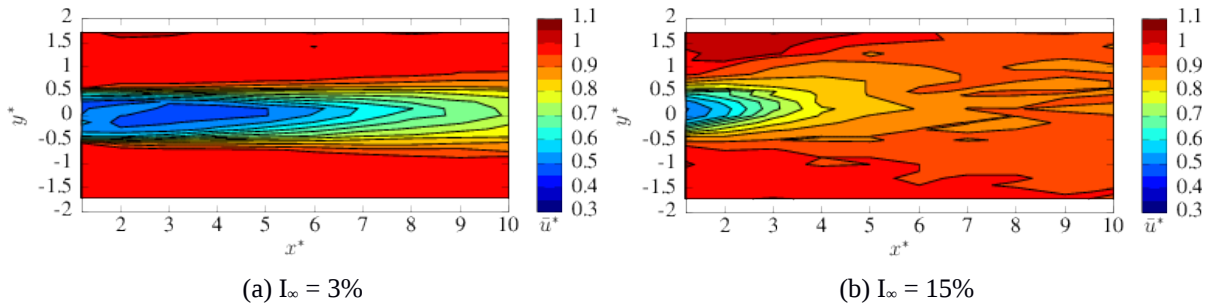
Fig. 1. Wake behind a turbine with TSR=3.67 , U_\infty=0.8 \text{ m.s}^{-1} for different ambient turbulences.
